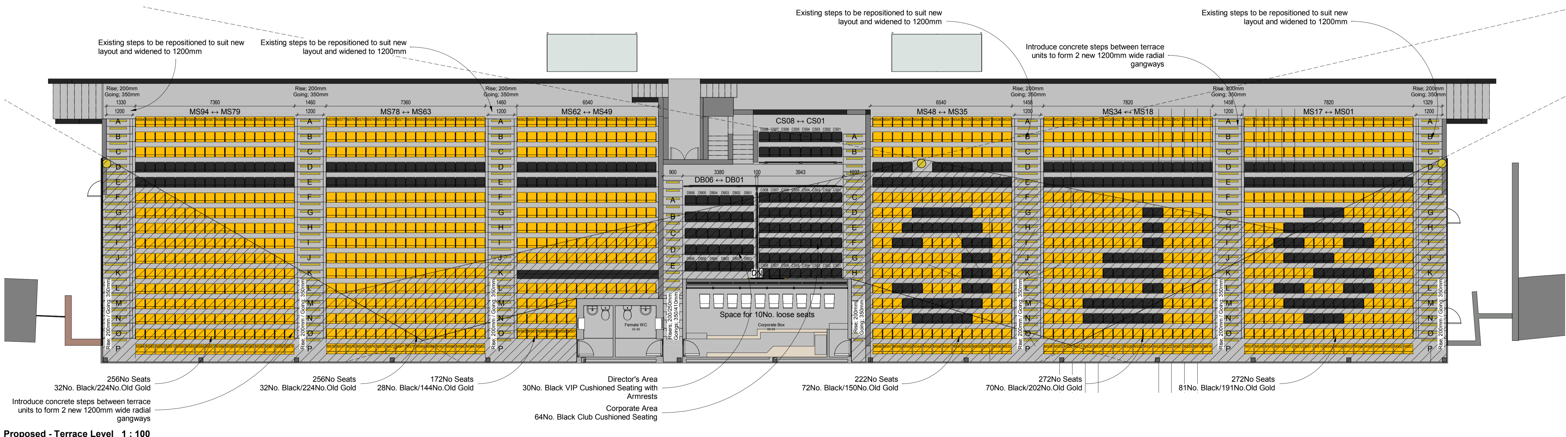
Proposed - Terrace Level 1 : 100
